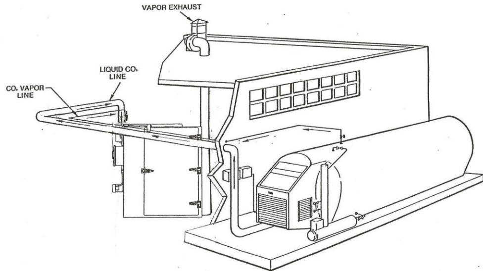
TYPICAL INSTALLATION CABINET FREEZER USING CO 2
